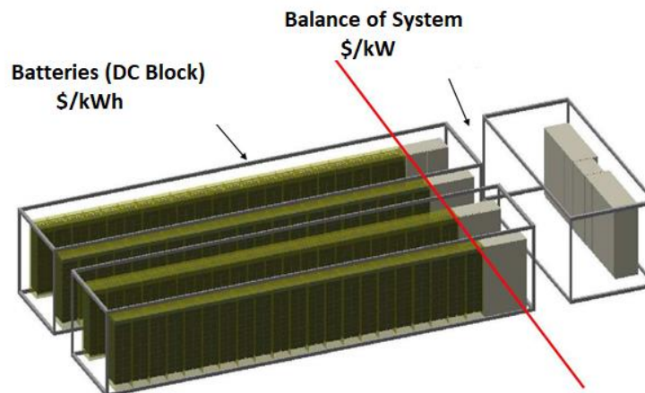
FIGURE 3.1 – Cost Components of a BESS
