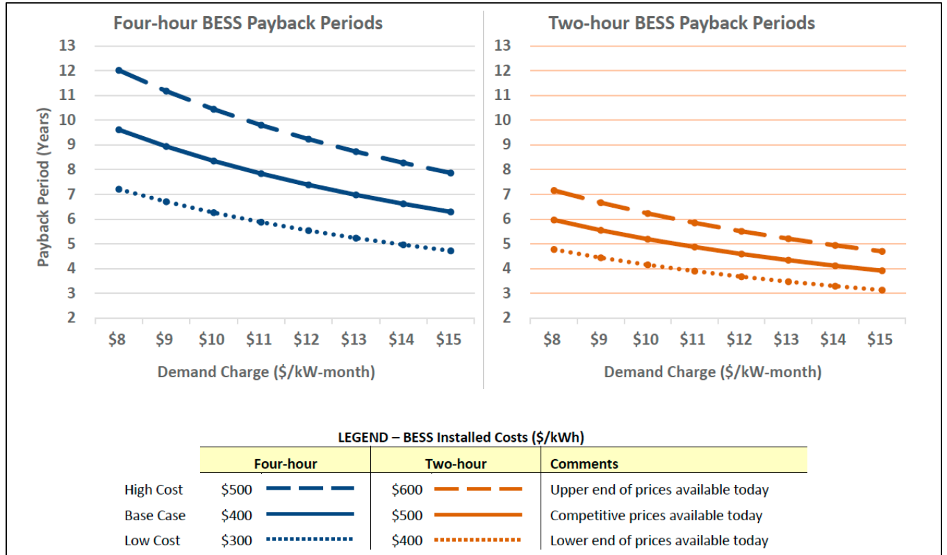
Figure 3.9: Payback Period for a 4-Hour and 2-Hour Battery Source: CFC
