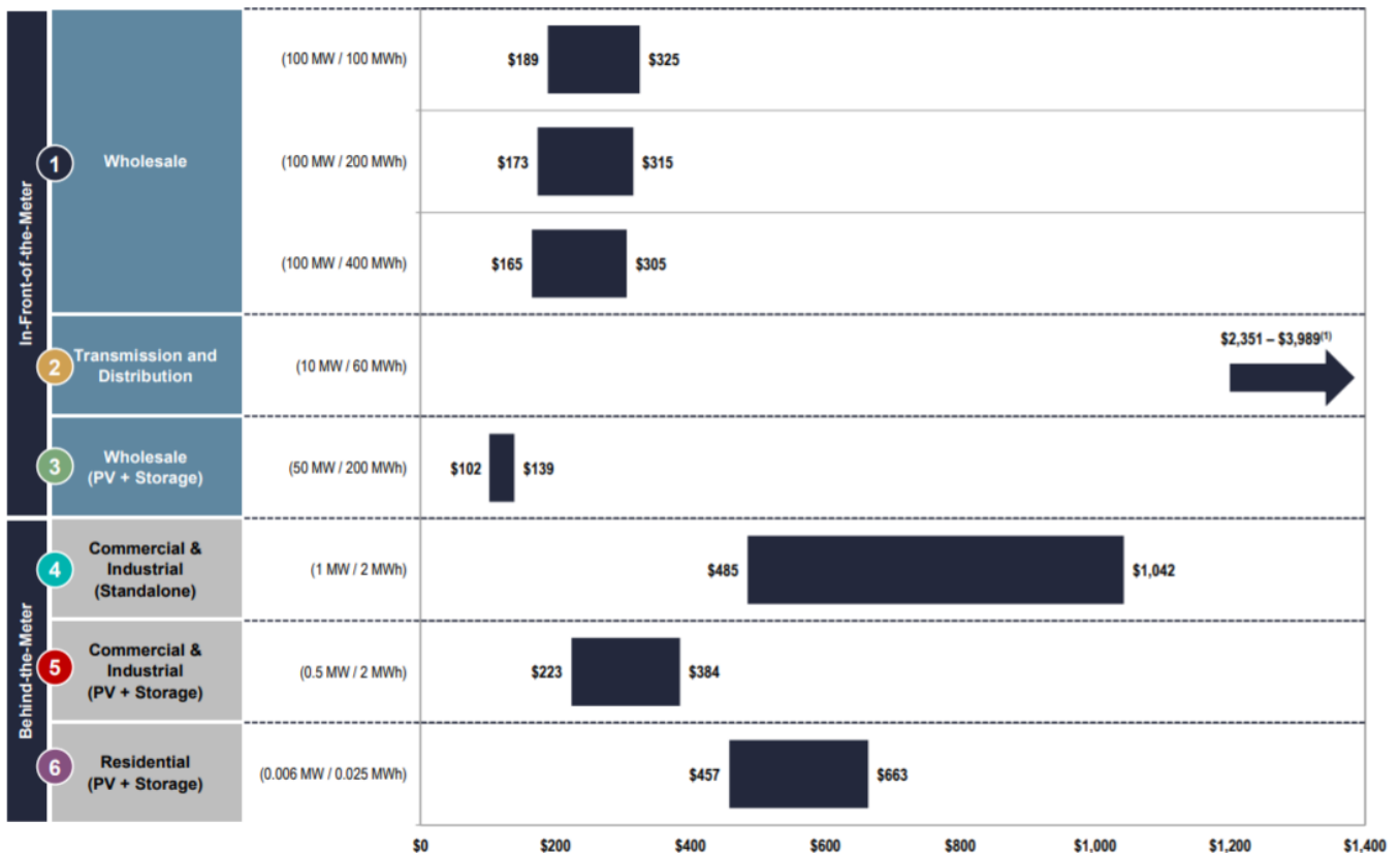
FIGURE 3.7 – Comparison of Unsubsidized LCOS ($/kW-year)
