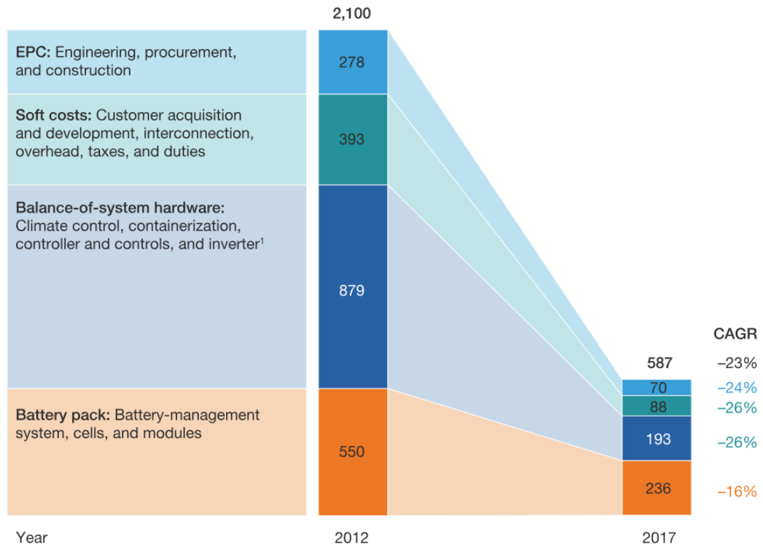
FIGURE 3.5 – Cost Breakdown of a 1 MWh BESS (2017 $/kWh)
