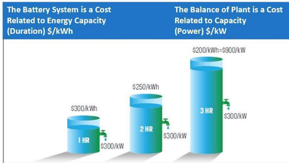
FIGURE 3.2 – Cost Components of a BESS Using a Water Tank as an Analogy
