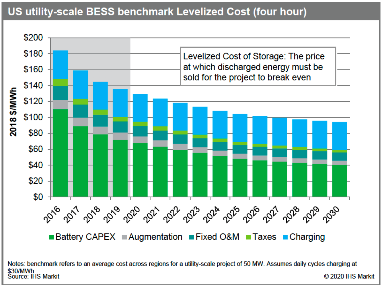
FIGURE 3.6 – Projected Cost Through 2030 ($/MWh)
