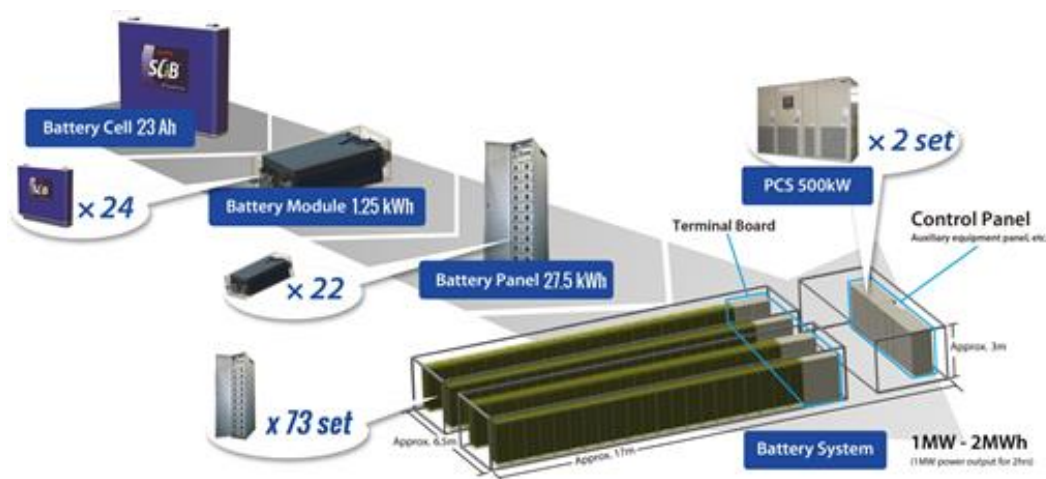
FIGURE 3.3 – Relationship Between Battery Cells, Modules and Panels
